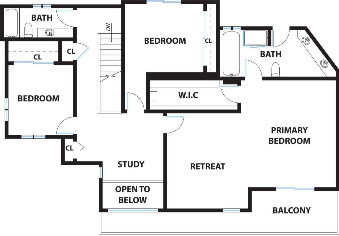
TOP LEVEL
